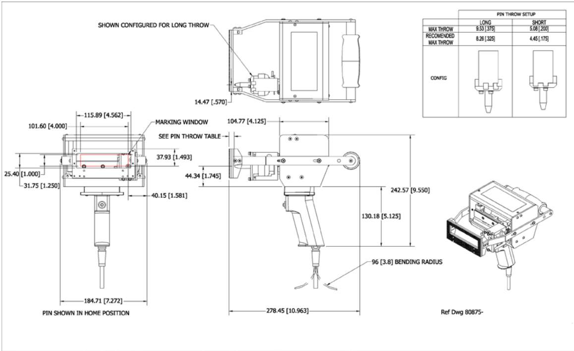
Nomad 4000 Hand-Held Marking Head Dimensions
